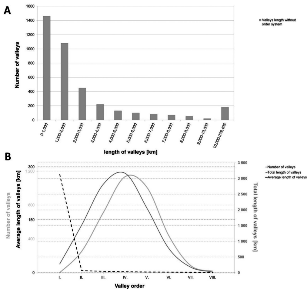
FIG. 2 - The number of all of the valleys in the Jemma River basin without using the Gravelius order system (a). The “number of valleys”, the “total length of valleys” and the “average length of valleys” of various orders in the Jemma River basin (according to the Gravelius order system of valley networks) (b).
