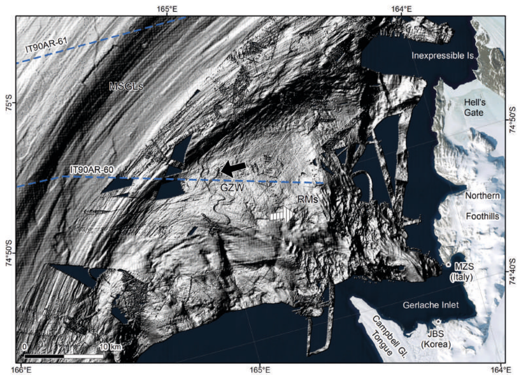
FIG. 6 - Detail of the Drygalski Basin Trough and of the Terra Nova Bay area (see fig. 2 for location). Morphobathymetric data compiled during the US cruises NBP0801, NBP1801, NBP1704 and the Italian OGS-PNRA cruise in the austral summer of 2005-06. Blue dashed lines indicate the seismic lines IT90AR_60 and IT90AR_61 (see fig. 2). MSGLs: mega-scale glacial lineations (LGM); GZW: grounding-zone wedge (ACR); the black arrow indicates ice-flow direction during ACR; RMs: recessional moraines; the white dashed arrow indicates mean receding ice flow direction. Satellite image Source: Esri, DigitalGlobe, GeoEye, Earthstar Geographics, CNES/Airbus DS, USDA, USGS, AeroGRID, IGN, and the GIS User Community.
