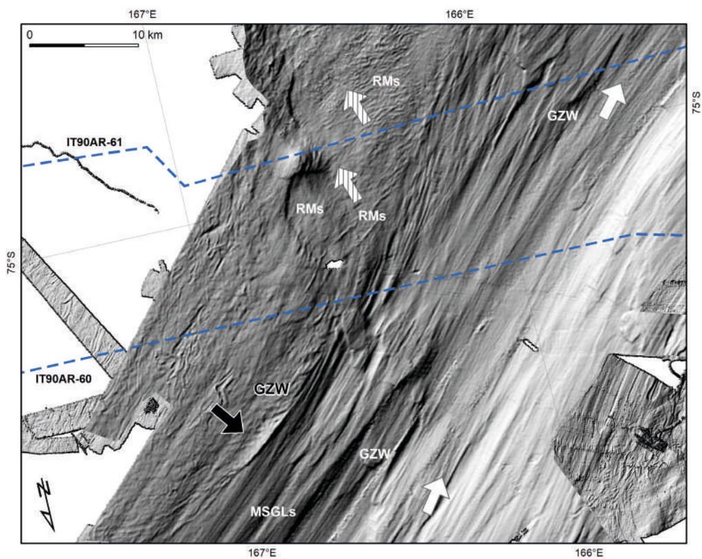
FIG. 7 - Detail of the Drygalski Basin Trough (see 2 for location). Morphobathymetric data compiled during the US cruises NBP0801, NBP1801, NBP1704 and the Italian OGS-PNRA cruise in the austral summer of 2005-06. Blue dashed lines indicate the seismic lines IT90AR_60 and IT90AR_61. The white arrow refers to the NNE-SSW oriented retreat of the marine-based Ross Ice Shelf (after the LGM); GZWs in white indicate stationary positions of the retreating ice sheet overlapping the previously scoured seafloor with mega-scale glacial lineations (MSGs, LGM). GZW in black and the black arrow show the ice-flow direction of an advanced phase of the ice sheet (ACR). White dashed arrows indicate the glacial retreat direction after the ACR, as underlined by recessional moraines (RMs) covering older seafloor features.
