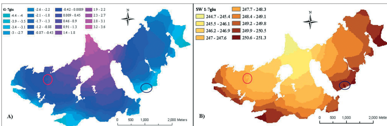
Fig. 6 - Example of maps representing temperature (A) and SWin (B) weekly distribution on Forni Glacier. Red circle marks the warmer island and the blue one indicates the colder island.
