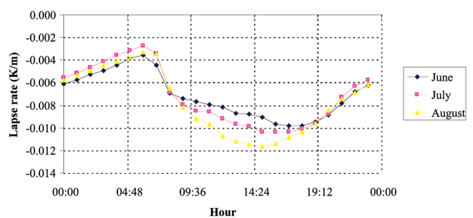
FIG. 4 - Hourly lapse rate between AWS S.Cat and AWS1 Forni averaged over the whole summer period 2009.
