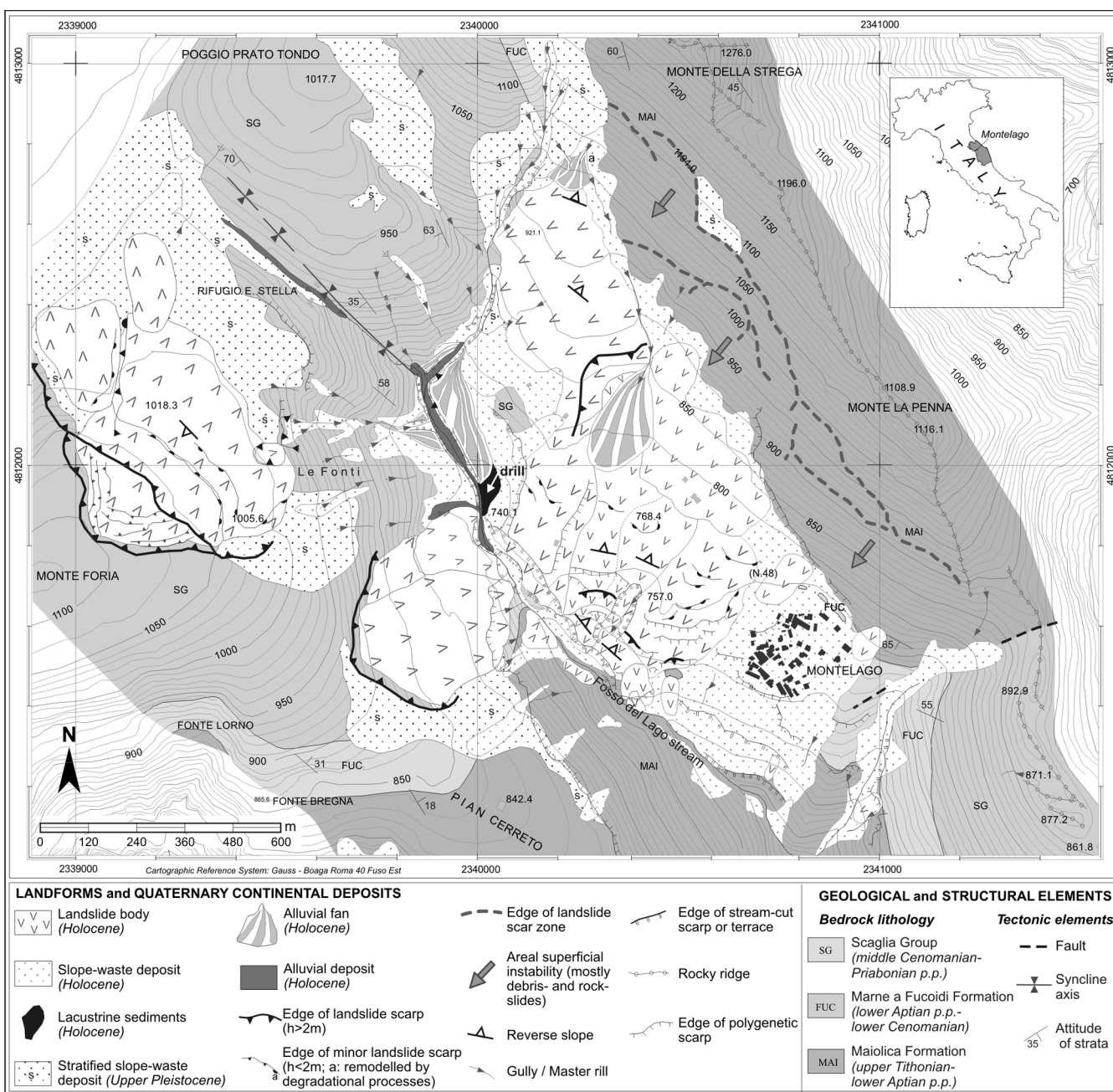
FIG. 2 - Geomorphological map of the Montelago area (after Savelli & alii, 2012, simplified).
