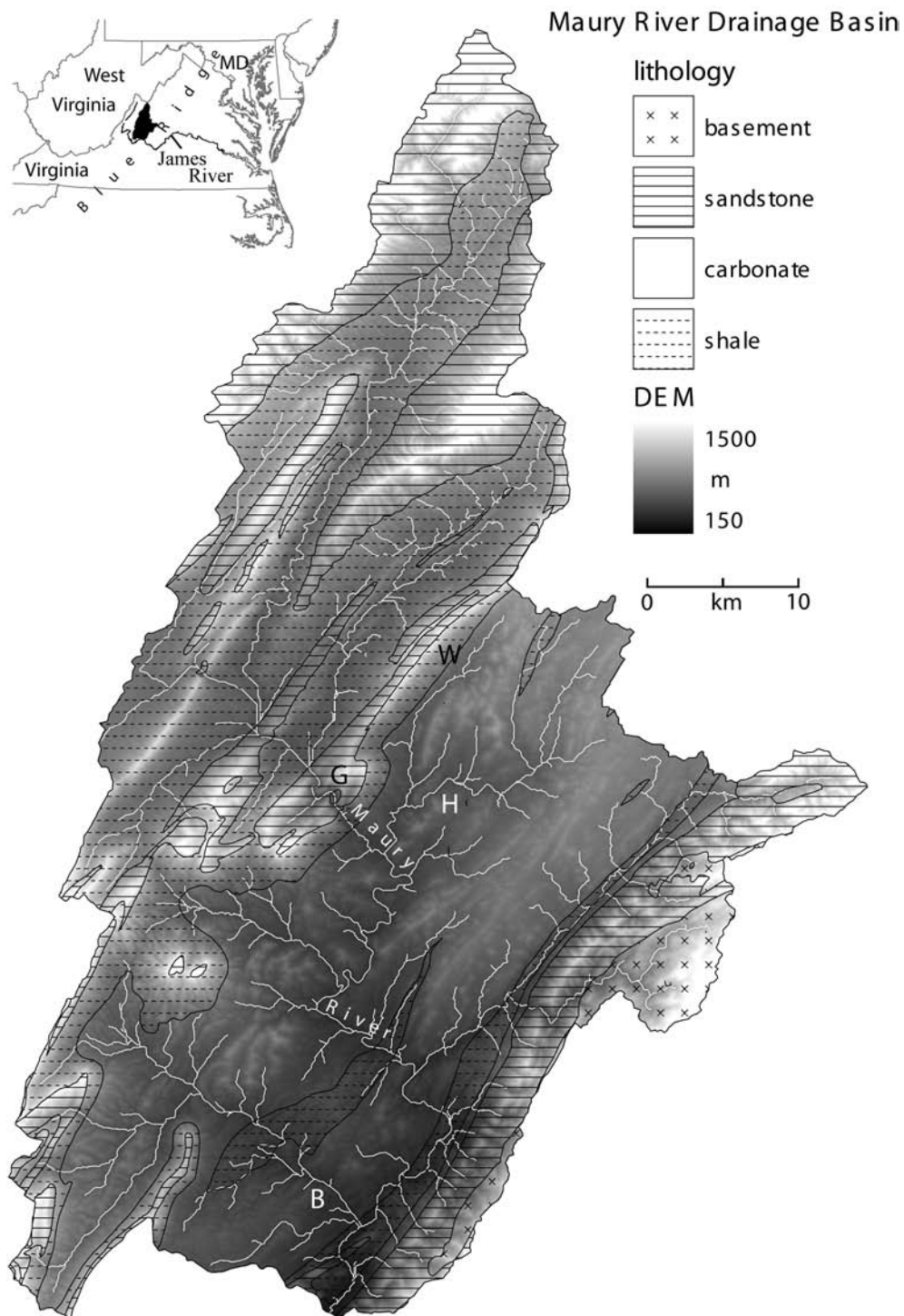
FIG. 1 - Location map showing topography (1° DEM), simplified geology (based on VDMR, 2003), DEM-derived drainage network (2.7 km 2 threshold), and locations discussed in the text; B - Buffalo Creek G - Goshen Pass water gap, H - Hayes Creek, W - Walkers Creek.
