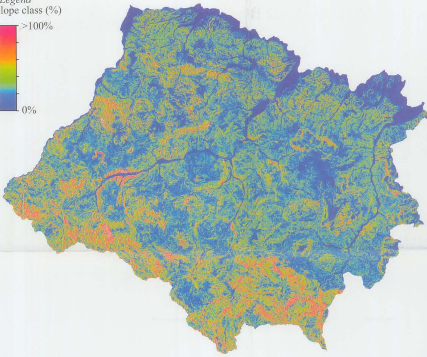
SLOPE MAP
