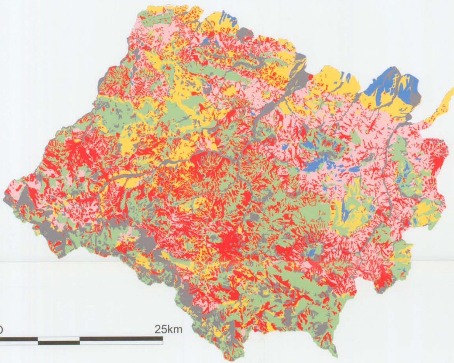
LITHOLOGICAL MAP
