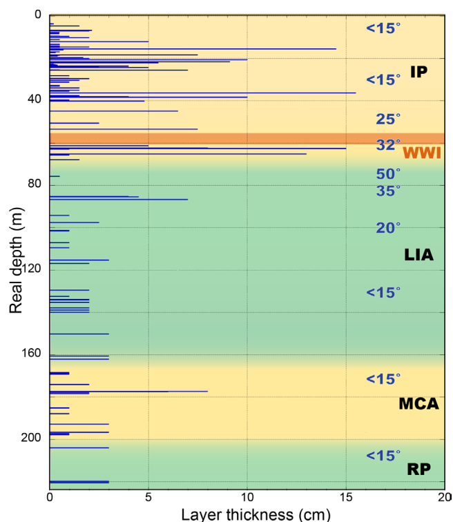
Figure 8 - Visual stratigraphy of ADA270 with dust layers thickness, tilting of the layers (only indicated in numerical form) and estimated age intervals. Layers with angle < 15^\circ are considered sub-horizontal. The depth of the various chronological intervals was calculated with the Dansgaard-Johnsen age model described in text. The orange bar represent the depth estimation of the World War I layers. (IP = Industrial Period; WWI = World War I; LIA = Little Ice Age; MCA = Medieval Climate Anomaly; RP = Roman Period).
