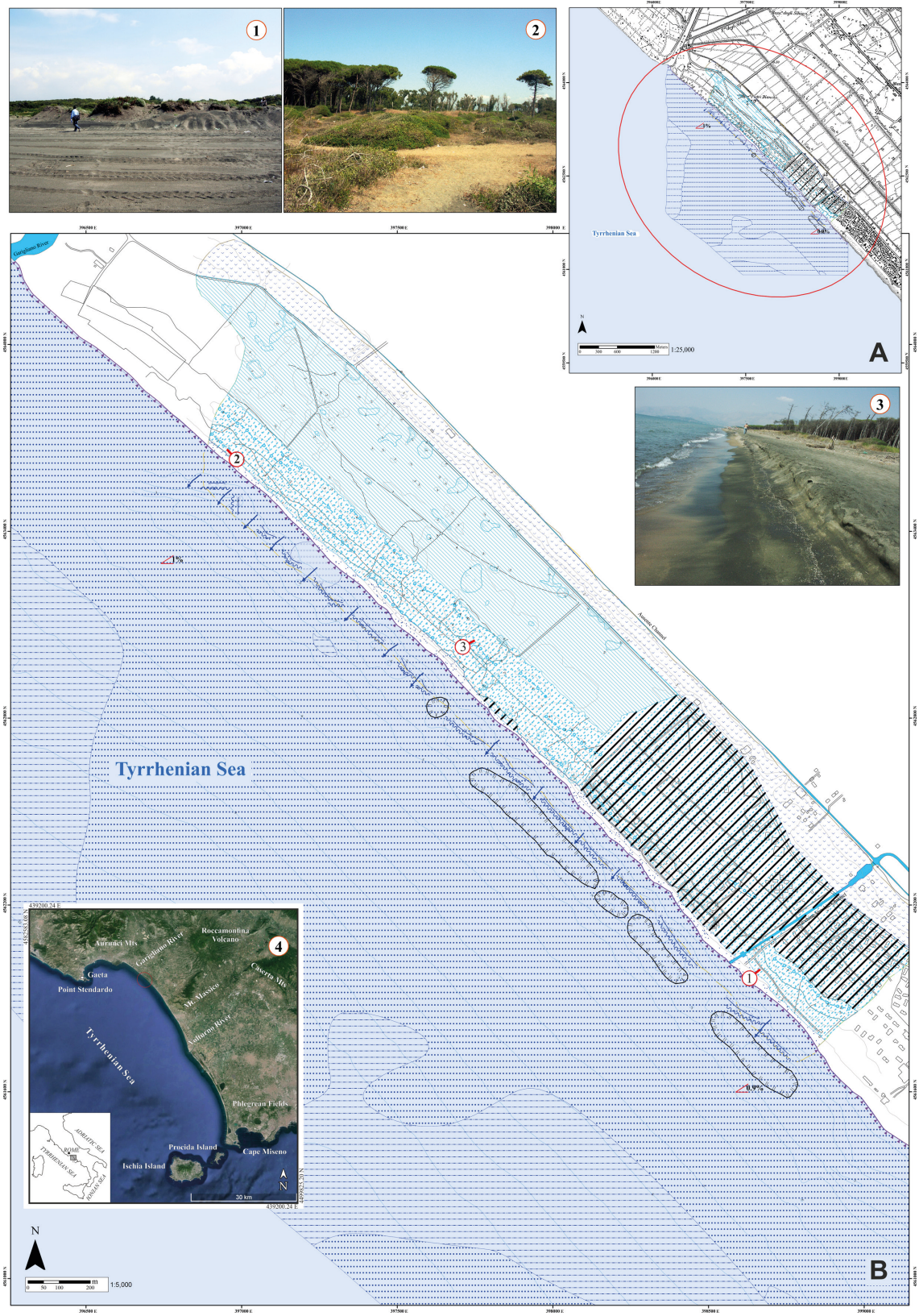
FIG. 10 - Geomorphologic maps of the SE of the Garigliano River Mouth (A, B): (1) anthropogenic remodeling of the beach due to cleaning and widening by mechanical vehicles; (2) blowout in the coastal dune modeled by wave erosion and airflow over the crest; (3) erosion scarp due to coastline retreat and consequent inland migration of beach-dune system; (4) coastal physiography of the Gulf of Gaeta. Circle in A indicates the location of the study area (B). See fig. 3 for legend.
