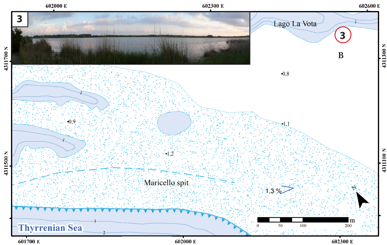
FIG. 11 - Geomorphologic maps of La Vota Paralic System (A, B): (1) the southern part of the Maricello spit; (2) the La Vota paralic system seen from Capo Suvero; (3) Lake La Vota, the innermost coastal basin of the La Vota paralic system. Circle in A represents the area enlarged in B. See fig. 3 for legend.
